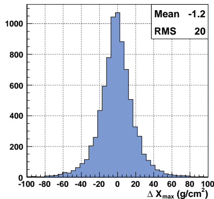
Figure 3: Resolution results for 10^{18} - 10^{19} eV ( E^{-2} differential spectrum). Applying cuts from [5], statistical resolution of 8% in energy and 20 \text{ g cm}^{-2} in X_{\max} is achieved.
