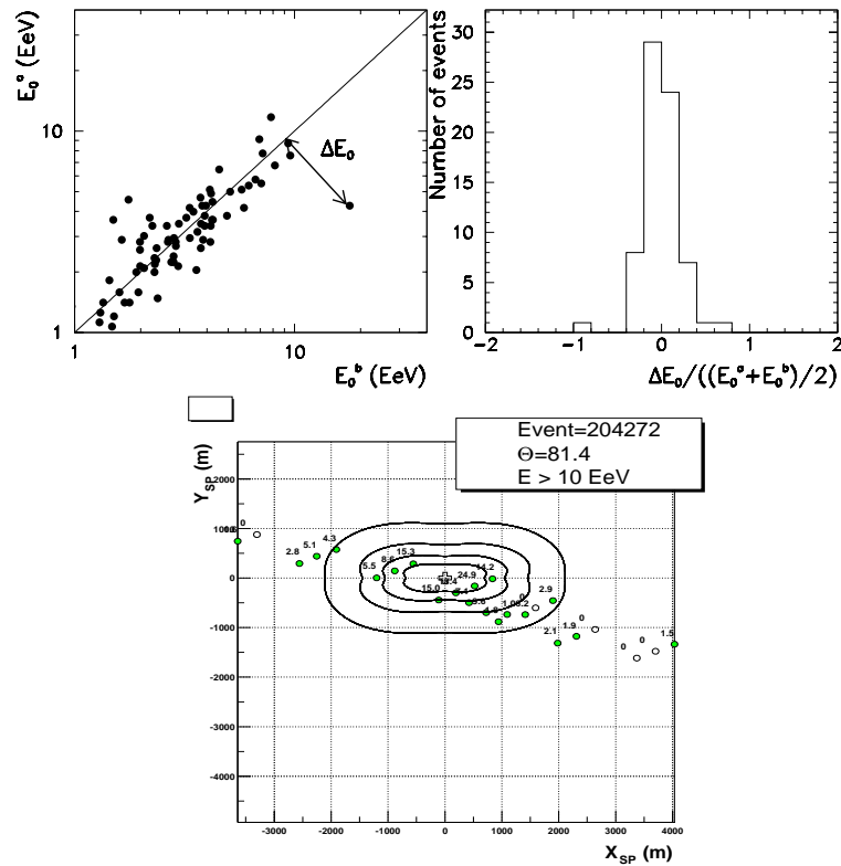
Fig. 1. Top left panel: Correlation of the reconstructed energy by two different algorithms, see text. Top right panel: Distribution of \Delta E_0 to the mean energy reconstructed by the two algorithms, see text. Bottom panel: Density map of an event, see text.
