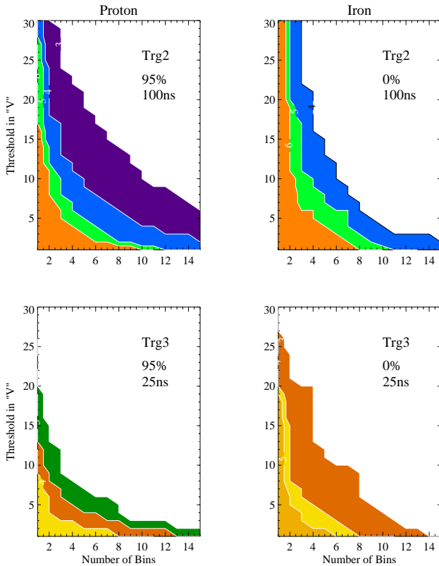
Fig. 3. Contour plots showing the number of triggered detectors per shower as a function of threshold (in 'V') and bin number for Proton and Iron showers. The Trg2 contours have 100ns wide bins, and the Trg3 contours have 25ns wide bins. The Proton 10^{19} eV contours are for a triggering efficiency of at least 95% and the Iron 10^{18} eV contours correspond to a triggering efficiency of 0%. Triggered detectors are represented in Trg2 by Purple (3), Blue (4), Green (5), and Orange (6); Trg3 by Green (2), Orange(3), Yellow (4).
