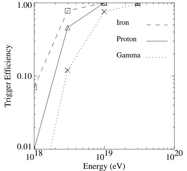
Fig. 4. Trigger Efficiency curves requiring a particular threshold of Trg2 and Trg3 and five or more detectors. Iron, Proton, and \gamma -induced shower sets are shown separately.
