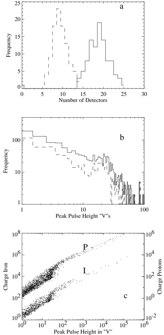
Fig. 2. (a) The distribution of ‘hit’ detectors before the trigger in a shower, the dashed line is for 10^{18} eV (Iron) events, the solid line for 10^{19} eV (Protons), (b) the peak pulse height distribution, the single muon peak is evident at approximately 20 ‘V’s, (c) the total charge in a detector FADC pulse vs the peak pulse height, the Protons are multiplied by 100 to separate them.
