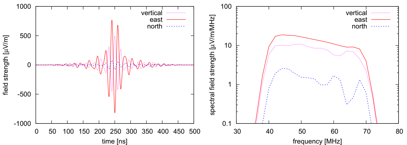
Fig. 11. Time traces (left) and frequency spectra (right) of the simulated event for the final, Hann-windowed three-dimensional electric field vector. The significant vertical component of the raw simulation has been reconstructed by the analysis chain. The final reconstructed arrival direction is \theta = 60.7^\circ and \phi = 295.1^\circ . The input direction for the simulated event was \theta = 58.4^\circ and \phi = 291.0^\circ . The frequency spectra correspond to the time traces shown here.
