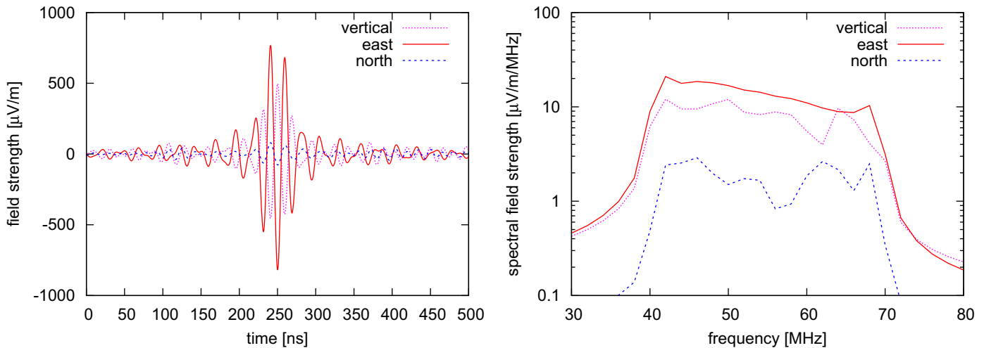
Fig. 10. Time traces (left) and frequency spectra (right) for the reconstructed three-dimensional electric field vector of the simulated event after application of the RdChannelWindowSetter . The leakage visible in the frequency spectra is due to the cutting of the time traces to a 500 ns window around the detected pulses. The frequency spectra correspond to the time traces shown here.
