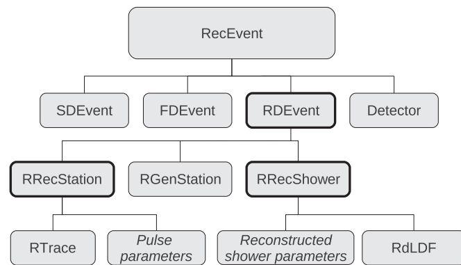
Fig. 4. Hierarchical structure of the radio-related quantities stored in ADST files. The individual classes constitute logical entities present in the Event data structures, storing for example information on Monte Carlo generated quantities in RGenStation and the reconstructed radio lateral distribution function in RdLDF .
