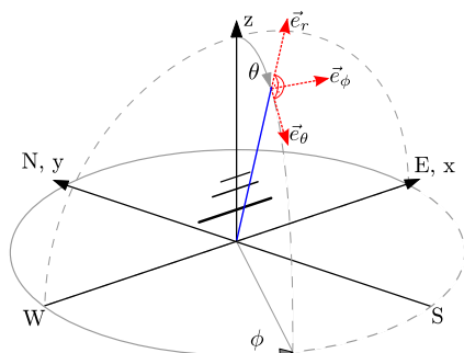
Fig. 3. The antenna characteristics are defined in a spherical coordinate system with the antenna in its center. The effective antenna height \bar{H}_{\text{eff}} for emission coming from a given arrival direction is decomposed into the components along the unit vectors e_\theta and e_\phi . These local (i.e., arrival direction-dependent) unit vectors lie in the plane perpendicular to the Poynting vector, which aligns with the dashed blue line in this figure for the incoming direction defined by \theta and \phi . As electromagnetic waves in air have no electric field component along the Poynting vector, this representation is complete. The antenna height itself is a frequency-dependent, complex quantity, the amplitude of which denotes the gain of the antenna, while the phase provides information about signal delays and dispersion. (For interpretation of the references to color in this figure legend, the reader is referred to the web version of this article.)
