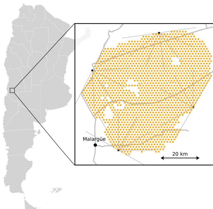
Figure 1. Layout of the Pierre Auger Observatory at Malargüe, Argentina. The position of the four FD buildings surrounding the SD array are indicated by the black squares, with gray lines indicating the field of view of the six telescopes at each building. Orange dots mark the position of each of the 1600 water-Cherenkov detectors, with a 1.5 km spacing between nearest neighbours.
